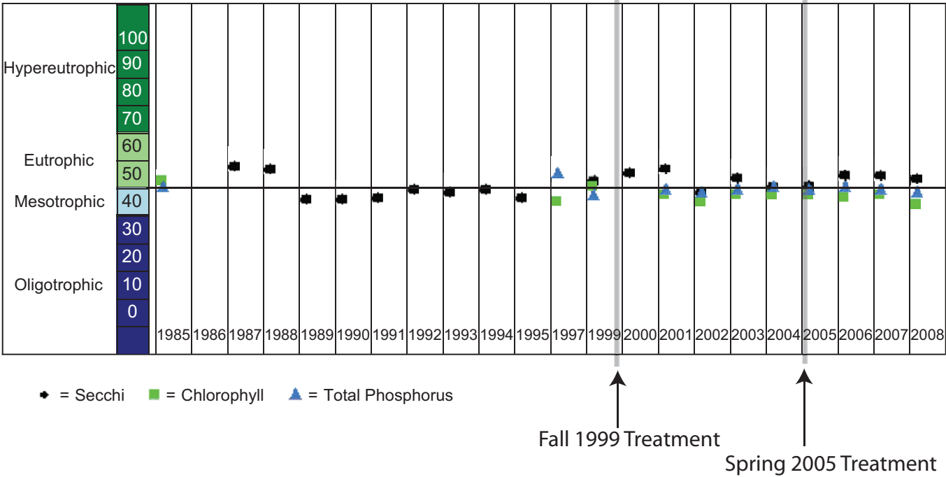
Graph 1 - Trophic State Index, Random Lake, 1985 through 2008.
